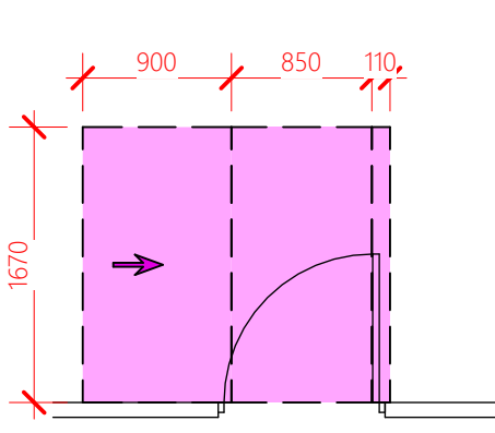
LATCH-SIDE APPROACH DOOR OPENS TOWARDS USER
