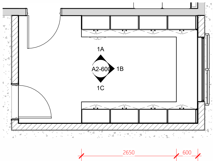
Internal Plan 1
