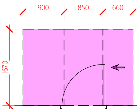
HINGE-SIDE APPROACH DOOR OPENS TOWARDS USER
