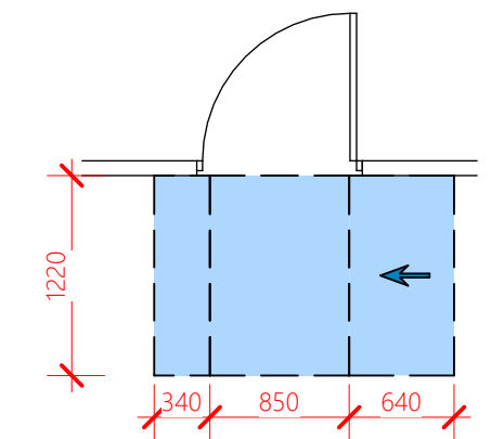
HINGE-SIDE APPROACH DOOR OPENS AWAY FROM USER
