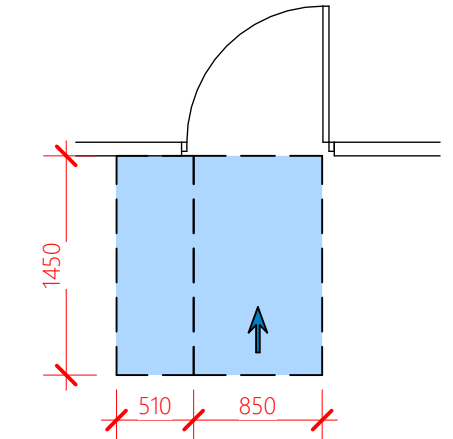
FRONT APPROACH DOOR OPENS AWAY FROM USER
