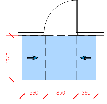
EITHER SIDE APPROACH DOOR OPENS AWAY FROM USER
