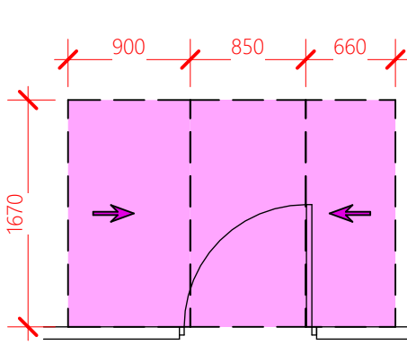
EITHER-SIDE APPROACH DOOR OPENS TOWARDS USER
