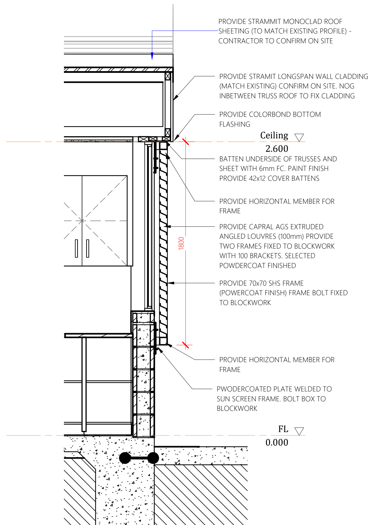
Section B1
