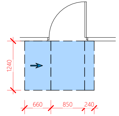
LATCH APPROACH DOOR OPENS AWAY FROM USER
