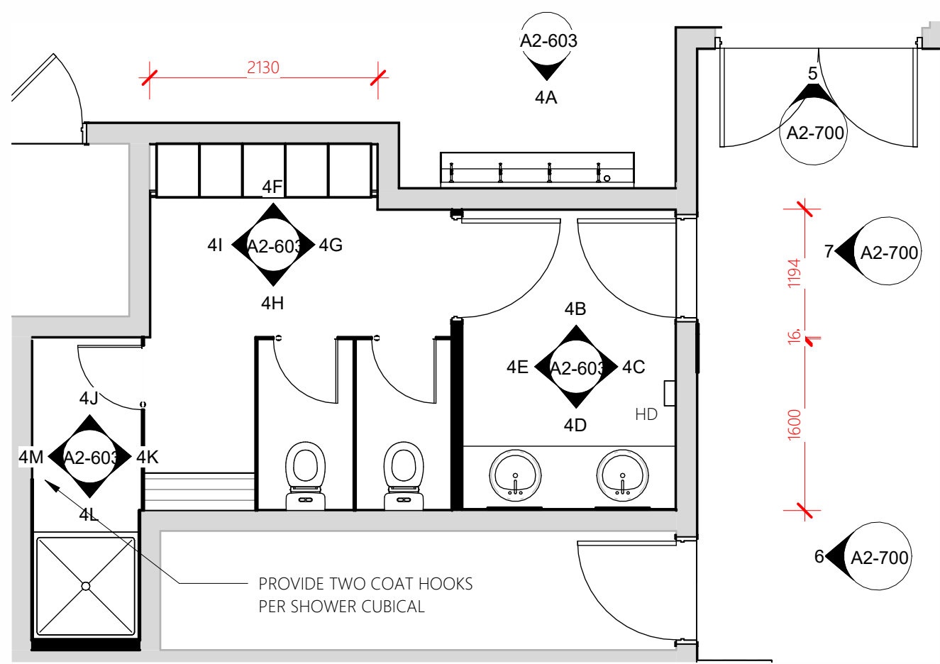
Joinery Plan 4
