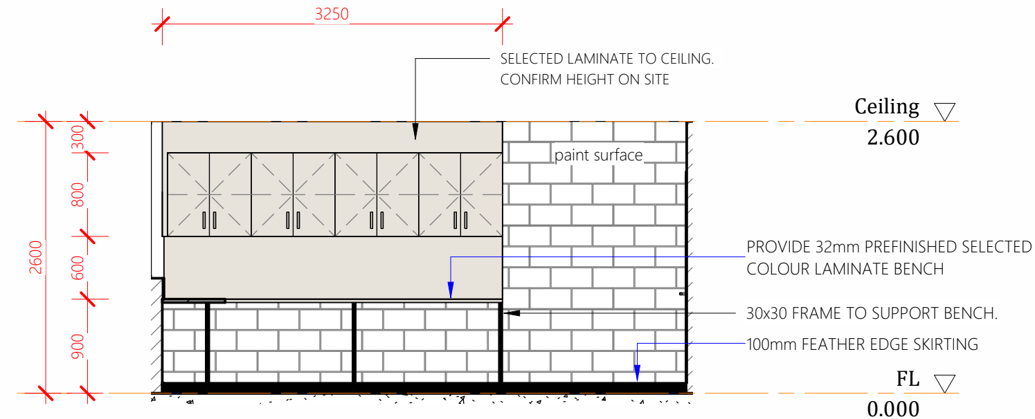
Elevation 1C
