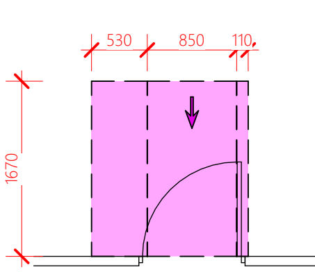
FRONT APPROACH DOOR OPENS TOWARDS USER
